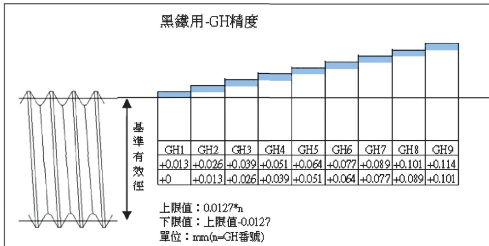
螺帽絲攻精度表
